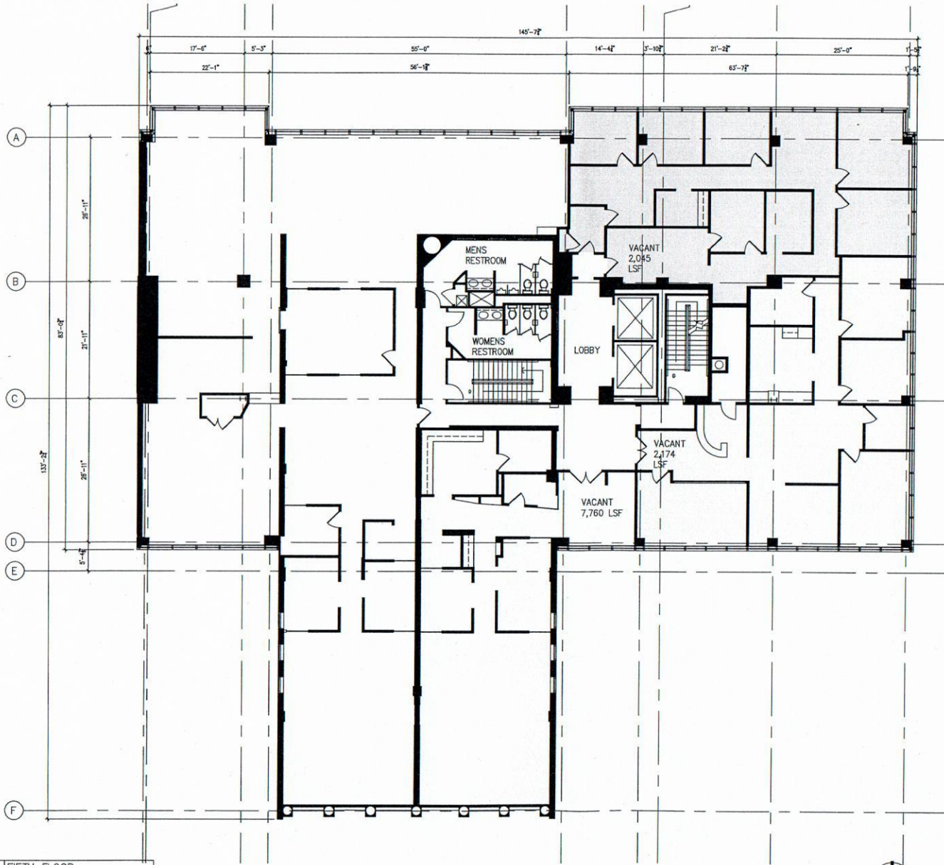
A1 FIFTH FLOOR EXISTING PLAN SCALE: 1/8"=1'-0"
